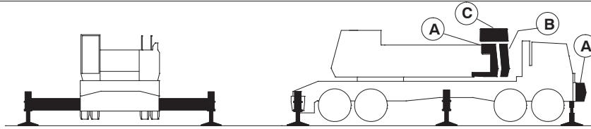
Main Boom Capacities – On Outriggers – 160 Ft Open Throat Tube Boom
