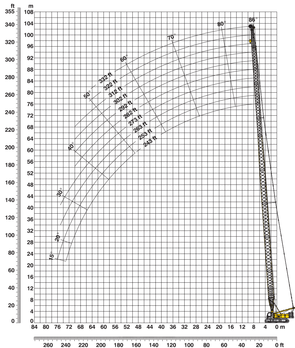
L-boom configuration with 168 ft main boom (No. 2018.xx/1713.xx) Configuration for L-boom lengths between 243 ft and 332 ft
