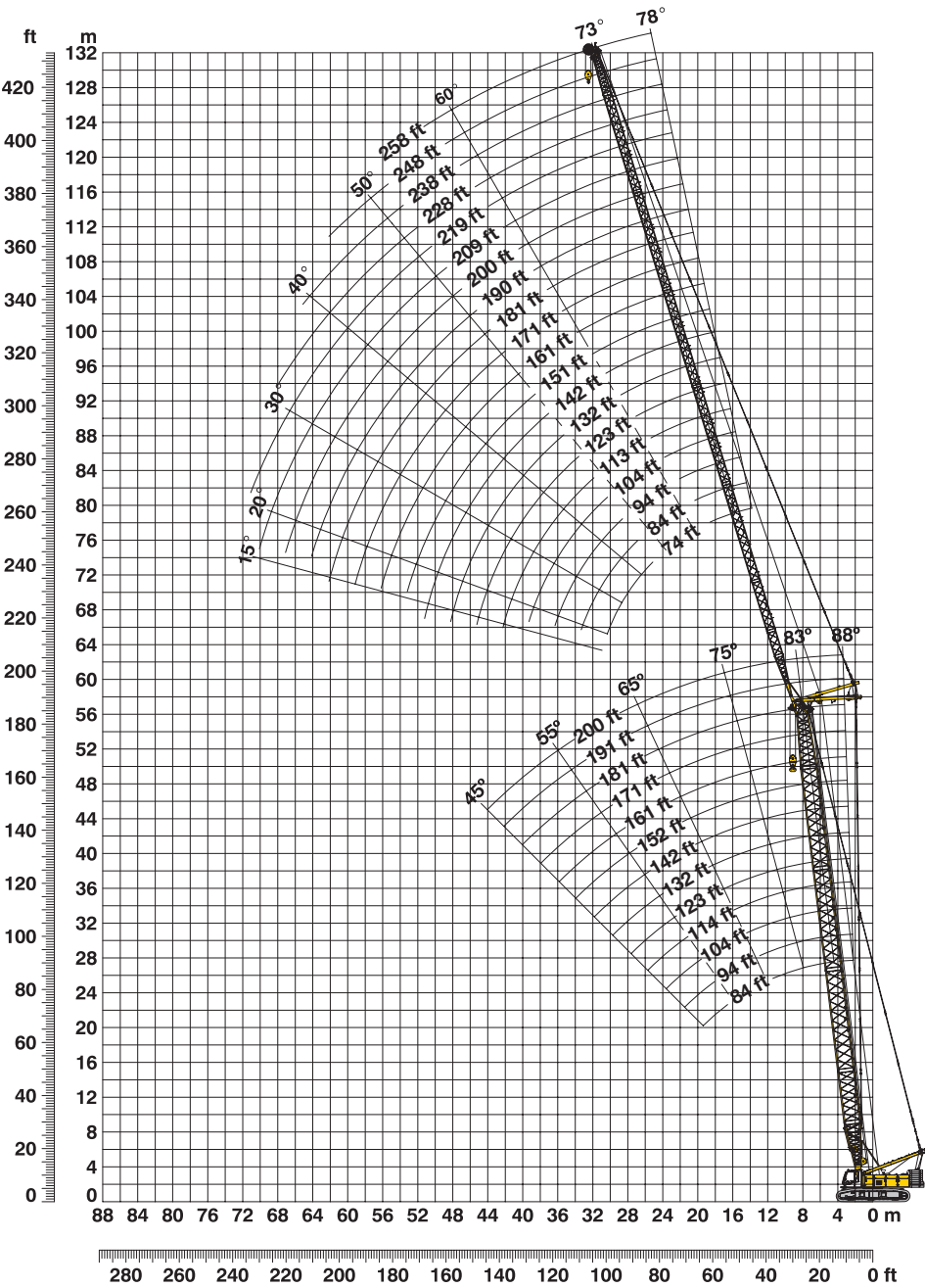
Boom configuration for main boom lengths (84 ft - 200 ft) – see table 1 on page 12 Jib configuration for jib lengths (74 ft - 258 ft)
