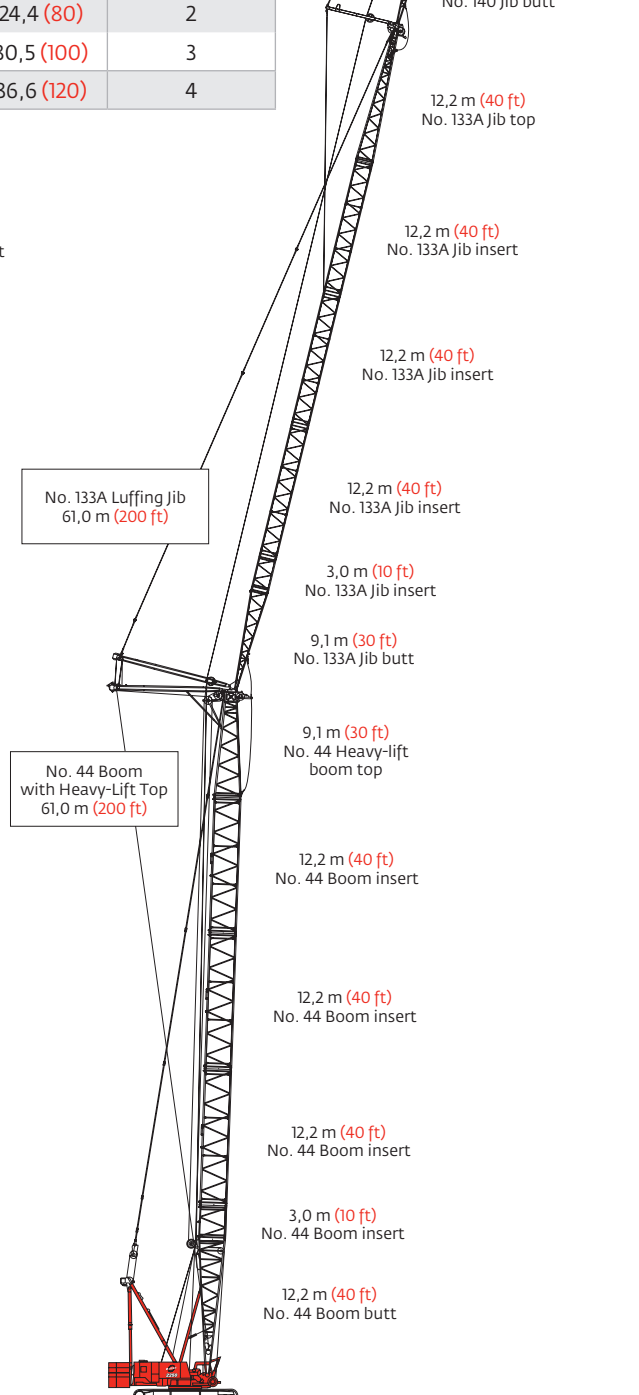
Model 2250 Series 3 No. 140 Fixed jib on No. 133A or No. 133 Luffing jib on No. 44 Main boom with heavy-lift top 158,5 m (520 ft)
