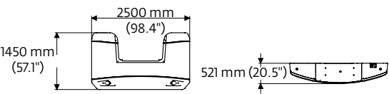
Rear counterweight
